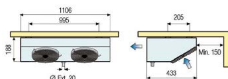
TN BT 009-016 009-012
